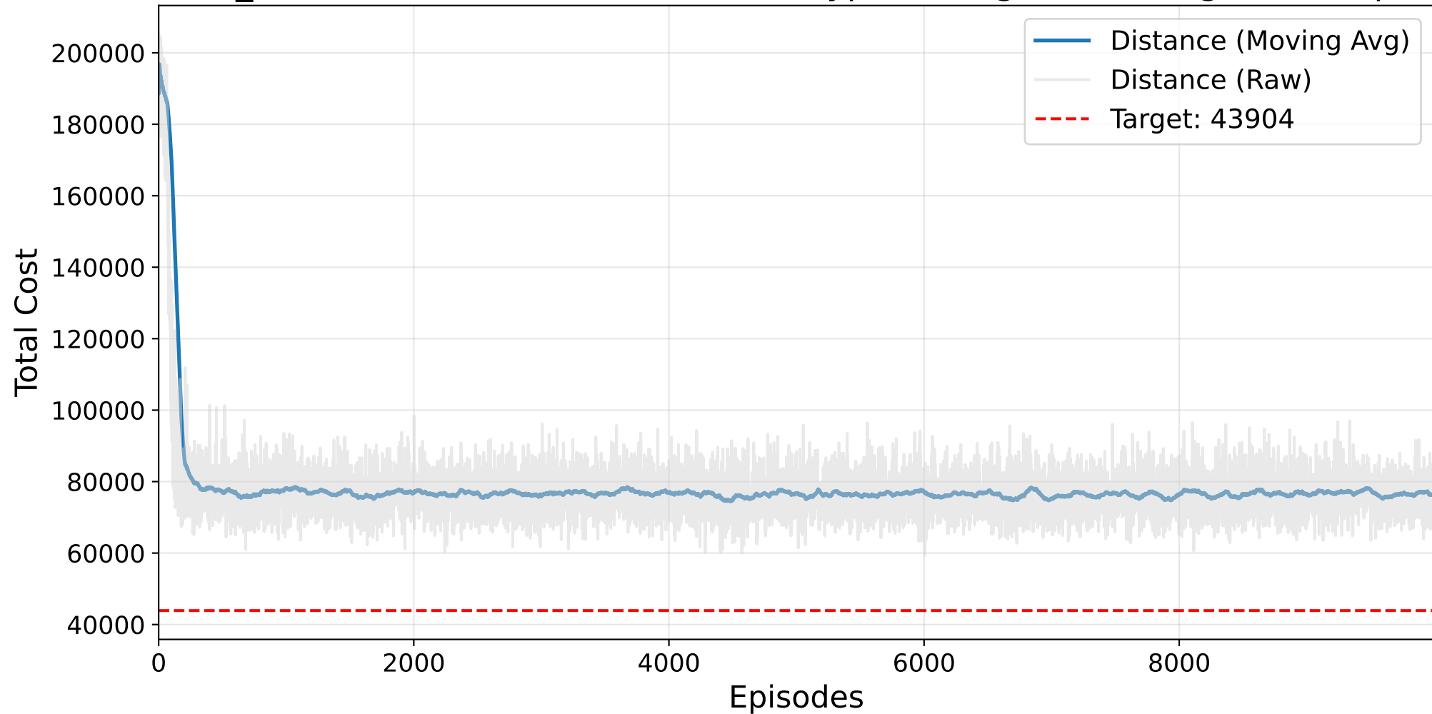
Final NO_BAYESIAN Masked AutoRL-SOP (HyperTuningSK) Training - kro124p.3.sop
